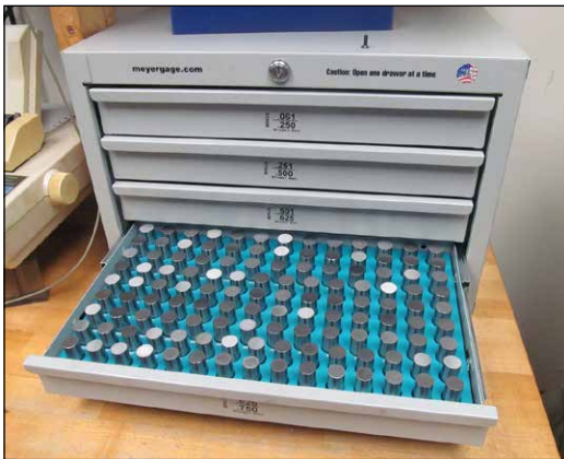
View of Pin Gage Sets
