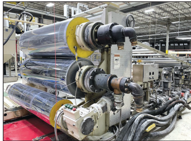
Chill Roll Polishing Stand, for PET Line
