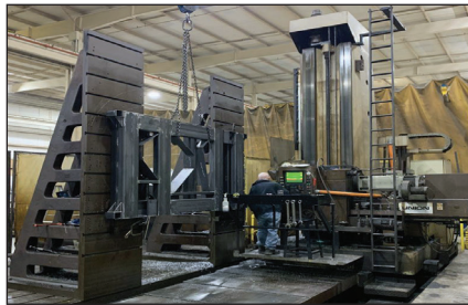
Union 6 in. BFP-130NC CNC Horiz. Floor Type HBM
